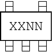
5-Lead SOT-23-5
