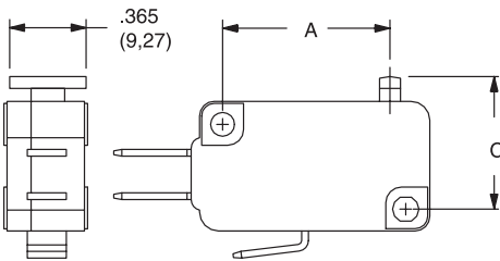
FIG. 5 Wide Pin
