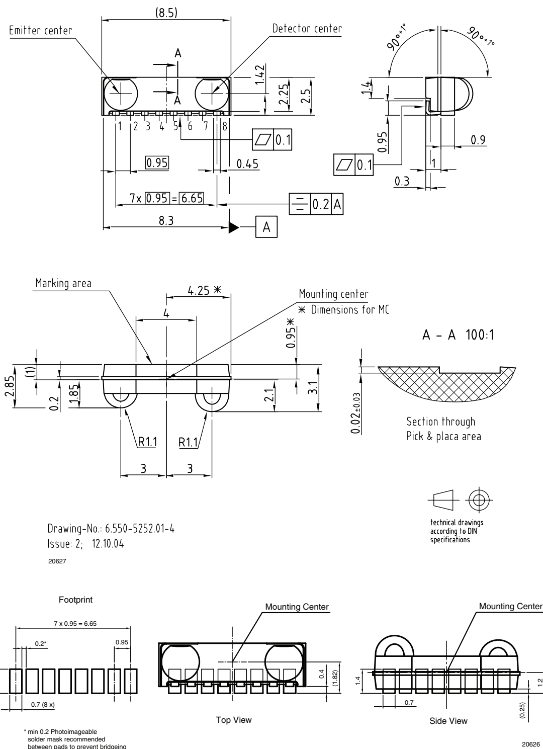
Figure 8. Package Drawing
