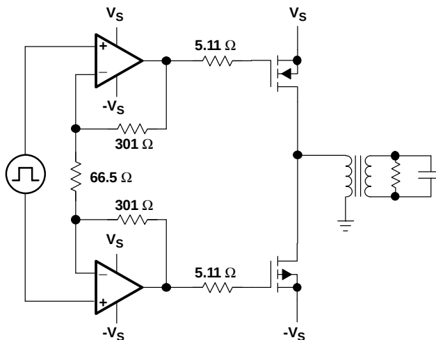
Figure 55. PowerFET Drive Circuit
