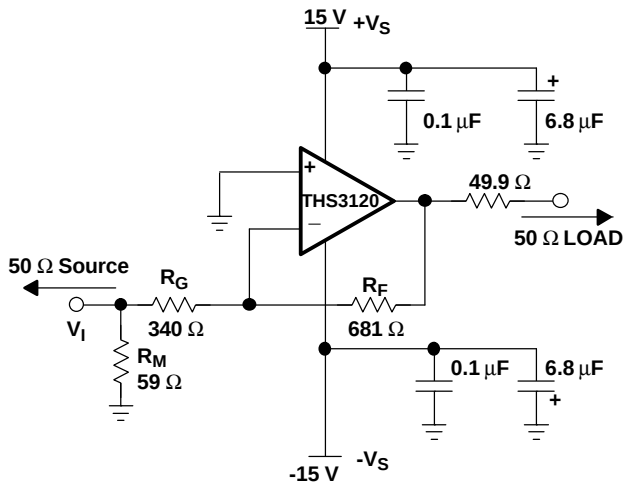
Figure 46. Wideband, Inverting Gain Configuration
