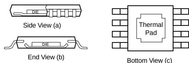
Figure 57. Views of Thermal Enhanced Package
