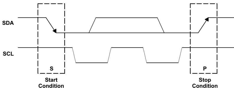
Figure 58. I 2 C Start and Stop Conditions
