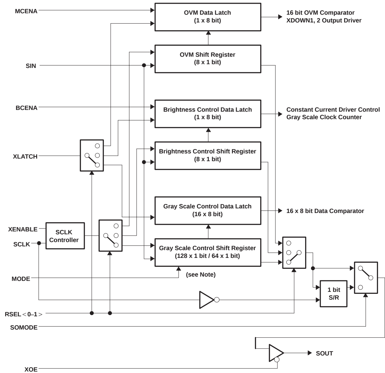
functional block diagram for shift register and data latch
