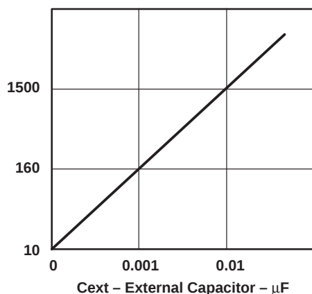
Figure 6. WDT Operational Time and Usage Example
