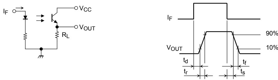
Note 3: Switching time measurement circuit and waveform
