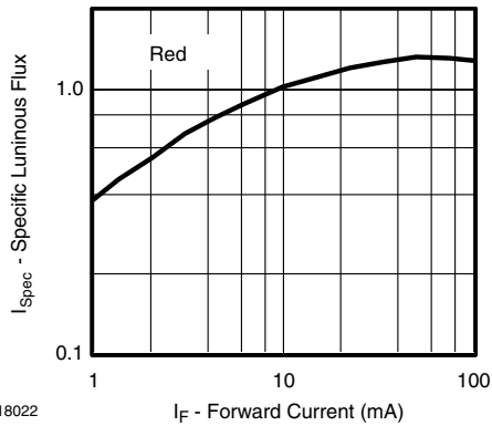
Figure 10. Specific Luminous Flux vs. Forward Current
