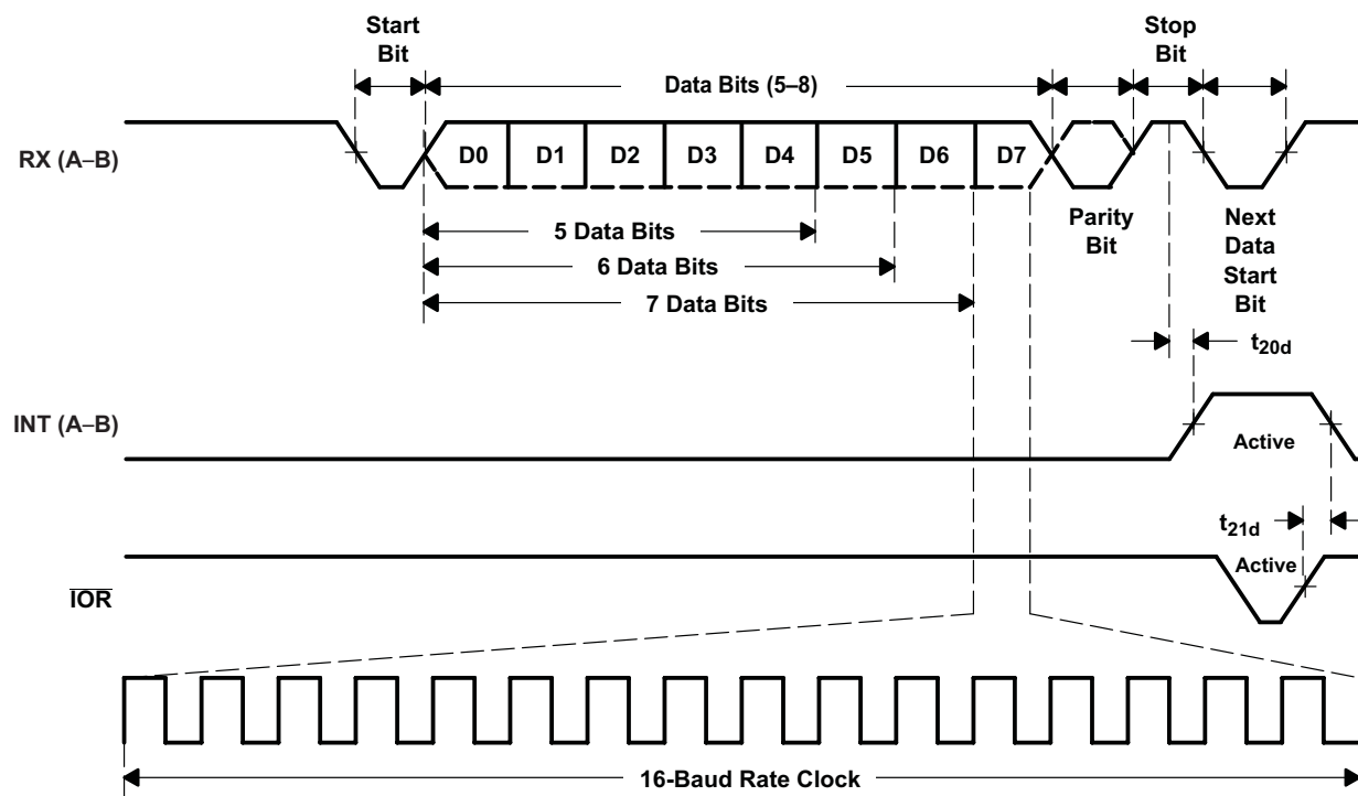
Figure 18. Receive Timing
