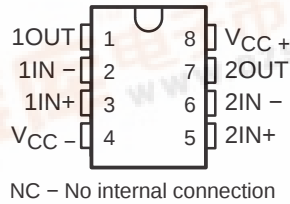
TL287, TL288 JG OR P PACKAGE (TOP VIEW)
