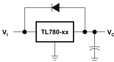
Figure 5. Reverse-Bias-Protection Circuit
