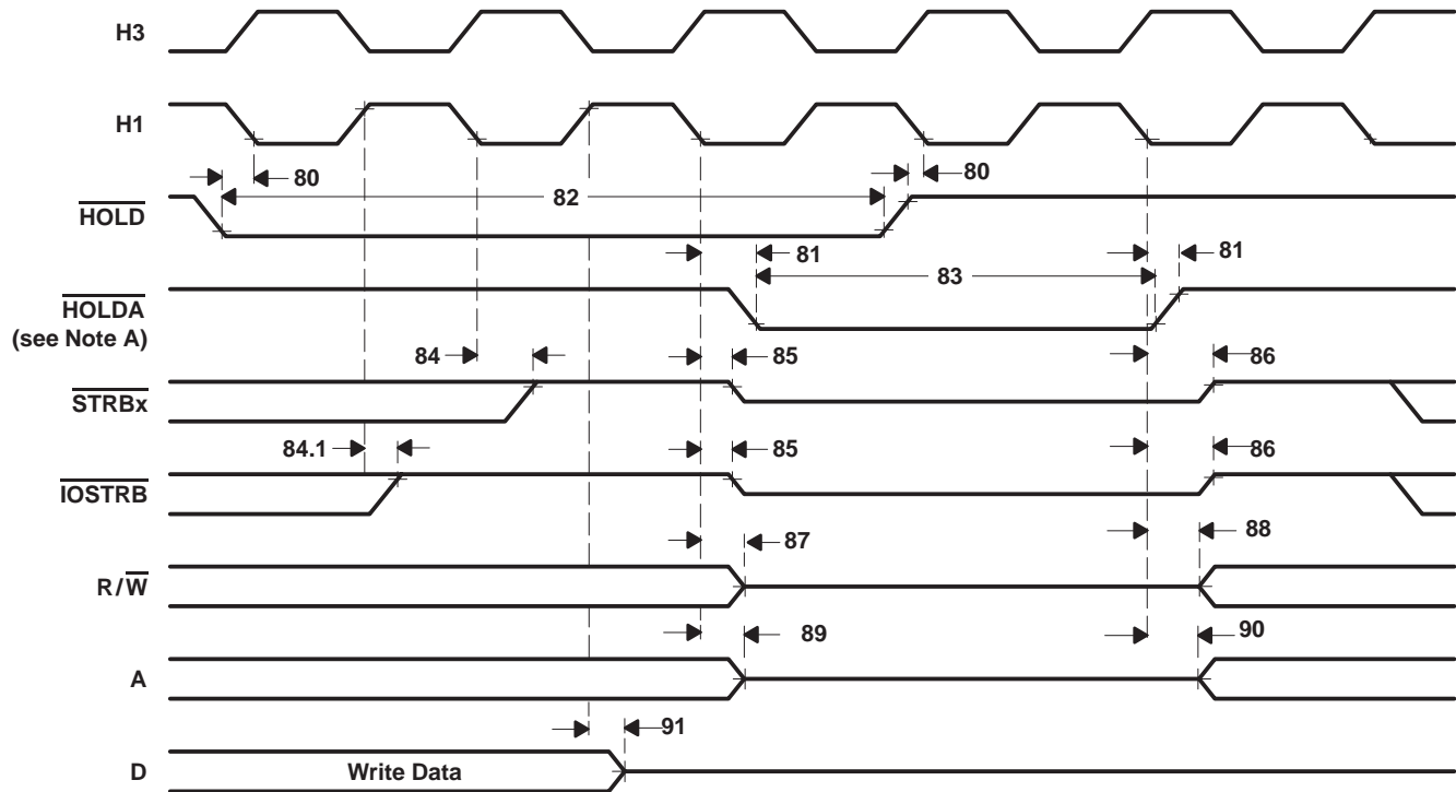
Figure 31. \overline{\text{HOLD}}/\overline{\text{HOLDA}} Timing
