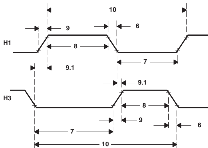
Figure 15. H1/H3 Timing
