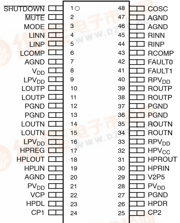
DCA PACKAGE (TOP VIEW)
