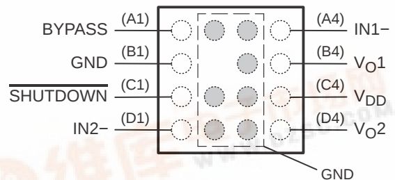
ZQY PACKAGE (TOP VIEW)
