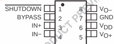
DGN Package (TOP VIEW)
