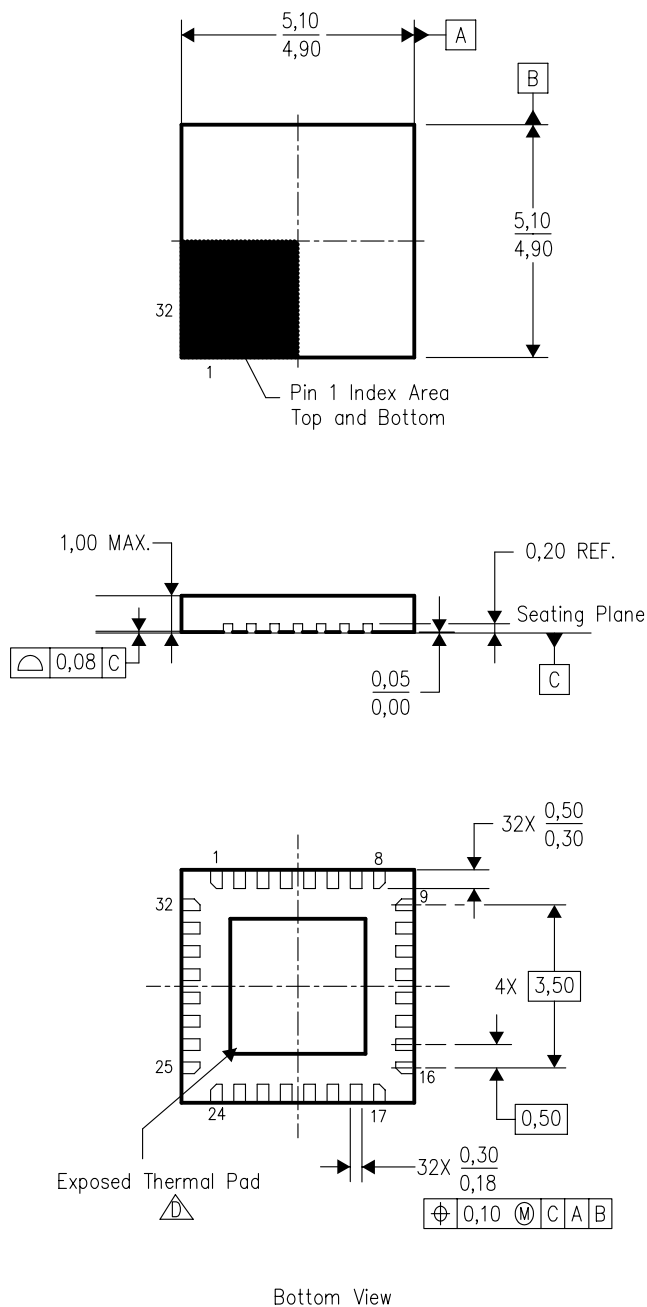
Bottom View
