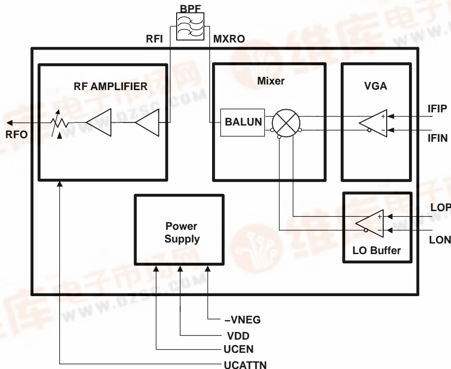
Figure 1. Block Diagram
