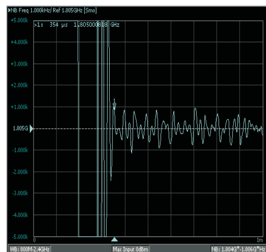
Figure 17. Frequency Locktime
