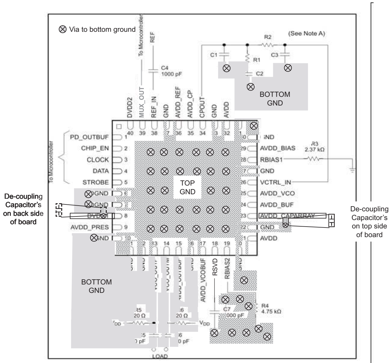
Figure 18. TRF3762 Layout
