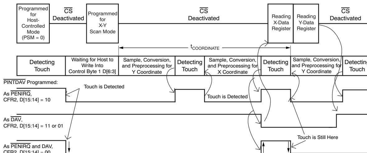
Figure 37. Example of an X and Y Coordinate Touch Screen Scan using TSMODE 2
