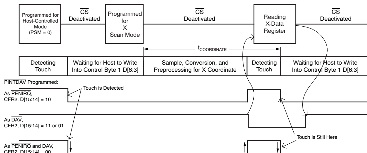
Figure 41. Example of a Single X Coordinate Touch Screen Scan (with Panel Stabilization Time) using TSMODE 3
