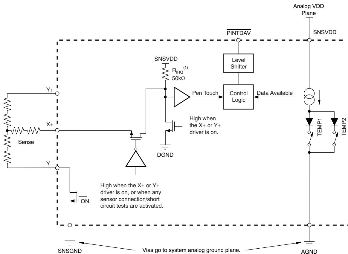
Figure 29. Example of a Pen-Touch Induced Interrupt via the PINTDAV Pin
