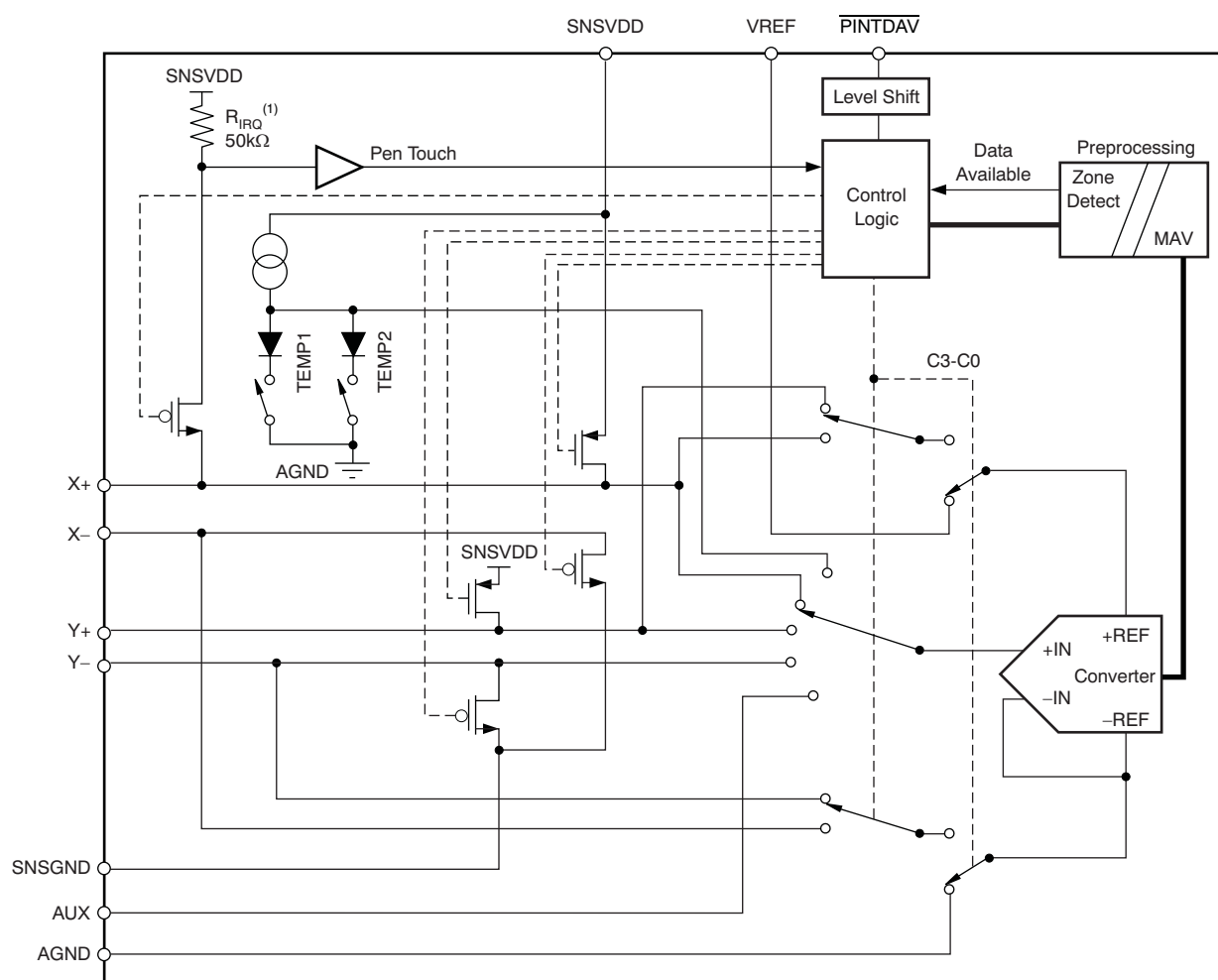
Figure 27. Simplified Diagram of the Analog Input Section
