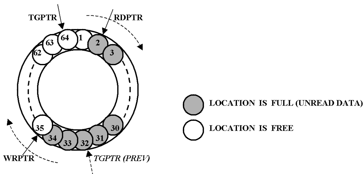
Figure 35. Circular Buffer
