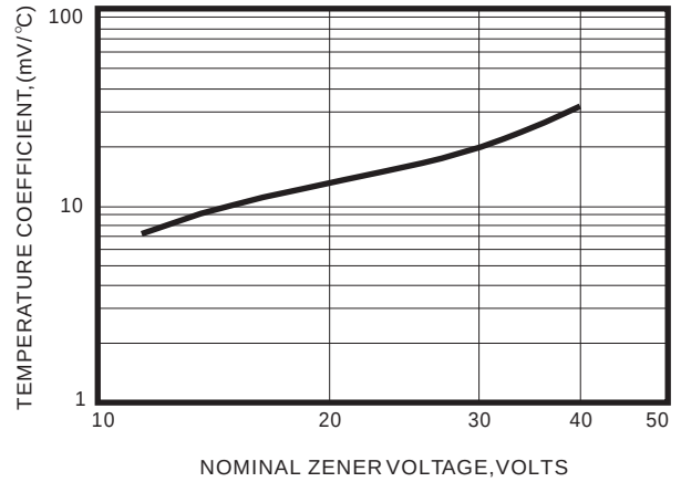
Fig.2 TEMPERATURE COEFFICENTS
