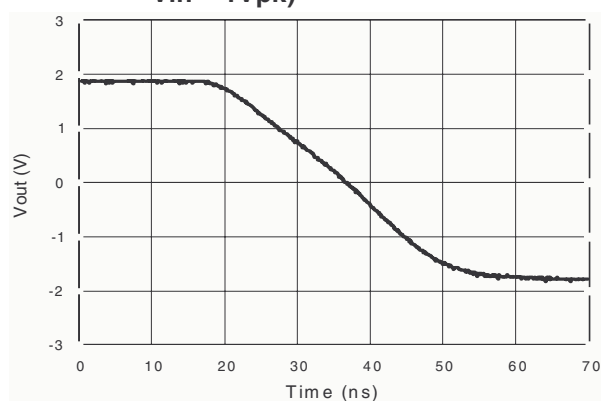
Figure 4. Large signal measurement - negative slew rate (Gain = 2, V_{CC} = \pm 2.5V , R_L = 150\Omega/5.6pF , V_{in} = 1V_{pk} )
