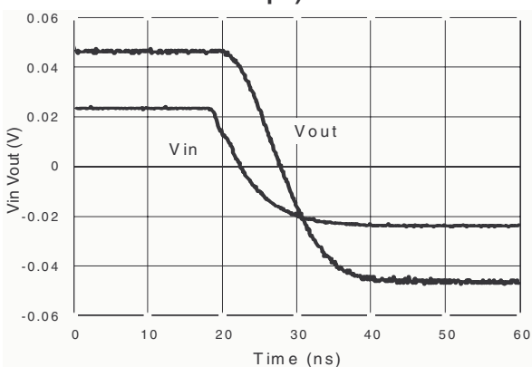
Figure 6. Small signal measurement - fall time (Gain = 2, V_{CC} = \pm 2.5V , Z_L = 150\Omega , V_{in} = 25mV_{pk} )
