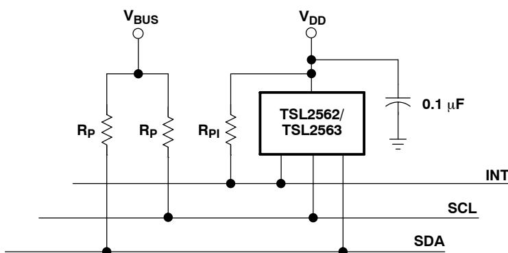
Figure 16. Bus Pull-Up Resistors
