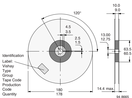
Figure 12. Dimensions of Reel
