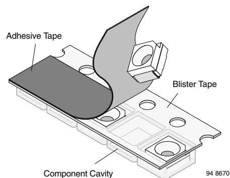
Figure 9. Blister Tape
