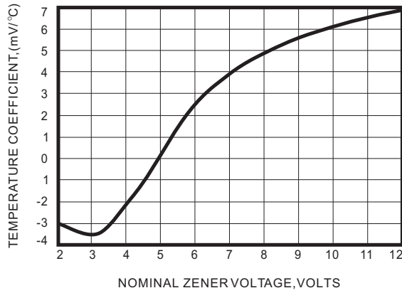
Fig.1 TEMPERATURE COEFFICENTS
