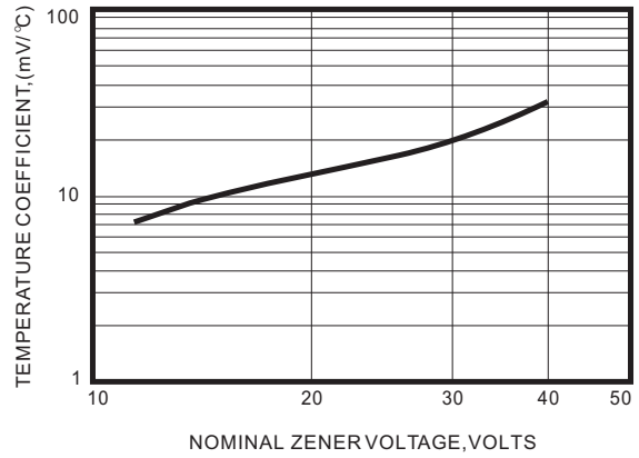
Fig.2 TEMPERATURE COEFFICENTS
