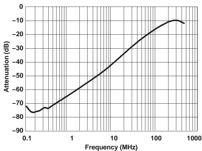
Figure 10. OFF Isolation vs Frequency ( V_+ = 5\text{ V} )
