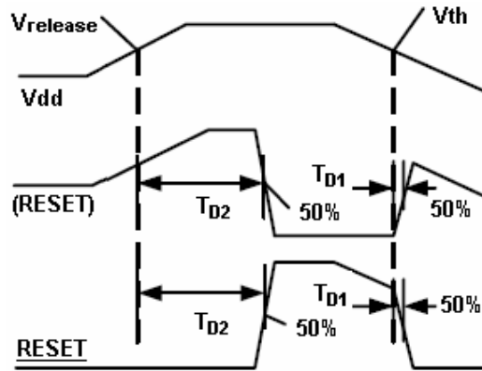
Reset Timing Diagram
