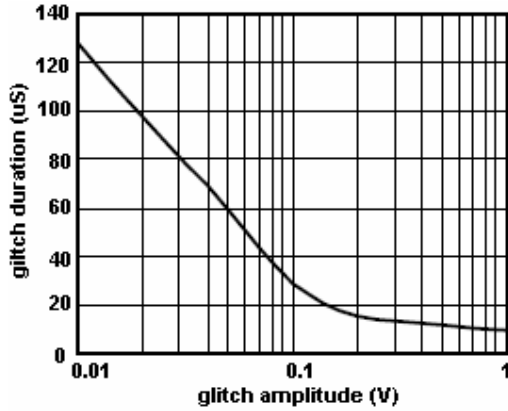
Fig 1. Glitch Rejection
