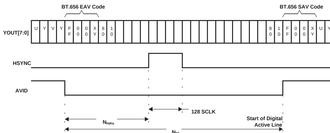
Figure 9-2. Horizontal Sync
