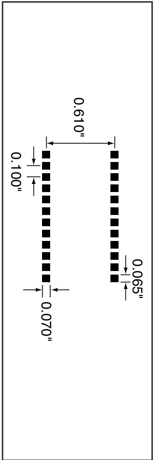
Figure 14: Recommended PCB Layout
