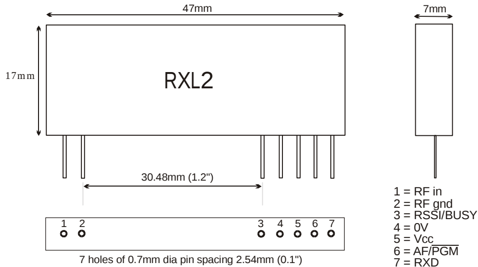
Figure 5: RXL2 footprint
