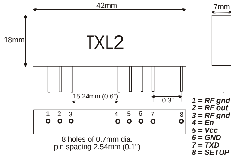
Figure 3: TXL2 footprint
