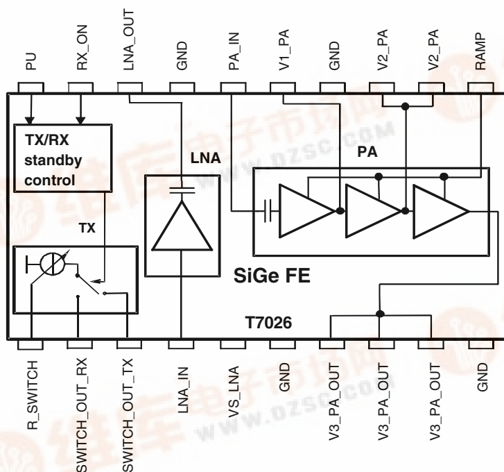
Figure 1-1. Block Diagram
