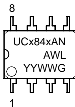
PDIP-8 N SUFFIX CASE 626
