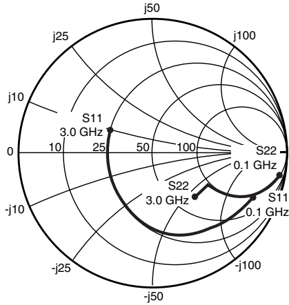
Coordinates in Ohms Frequency in GHz V CE = 5 V, I c = 5 mA Z 0 = 50 Ω
