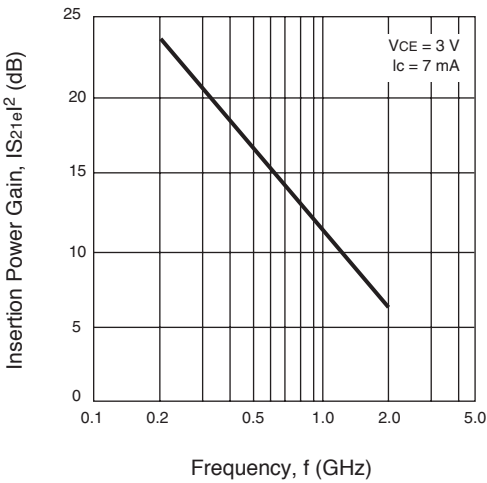
INSERTION POWER GAIN vs. FREQUENCY
