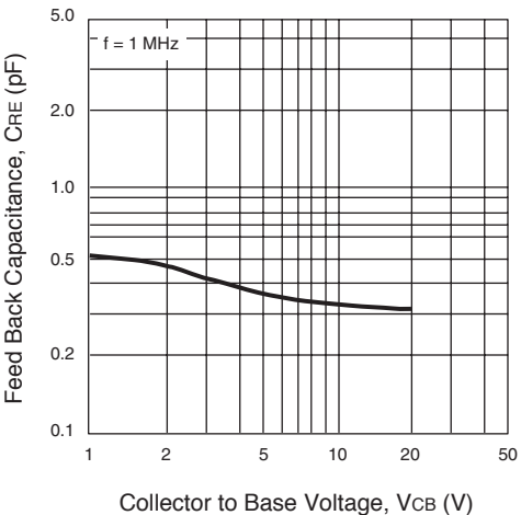
FEED BACK CAPACITANCE vs. COLLECTOR TO BASE VOLTAGE
