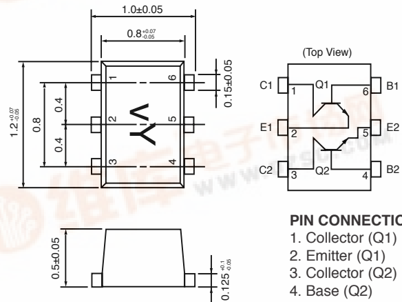
Package Outline TD (TOP VIEW)
