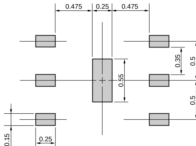
SOLDER PAD
