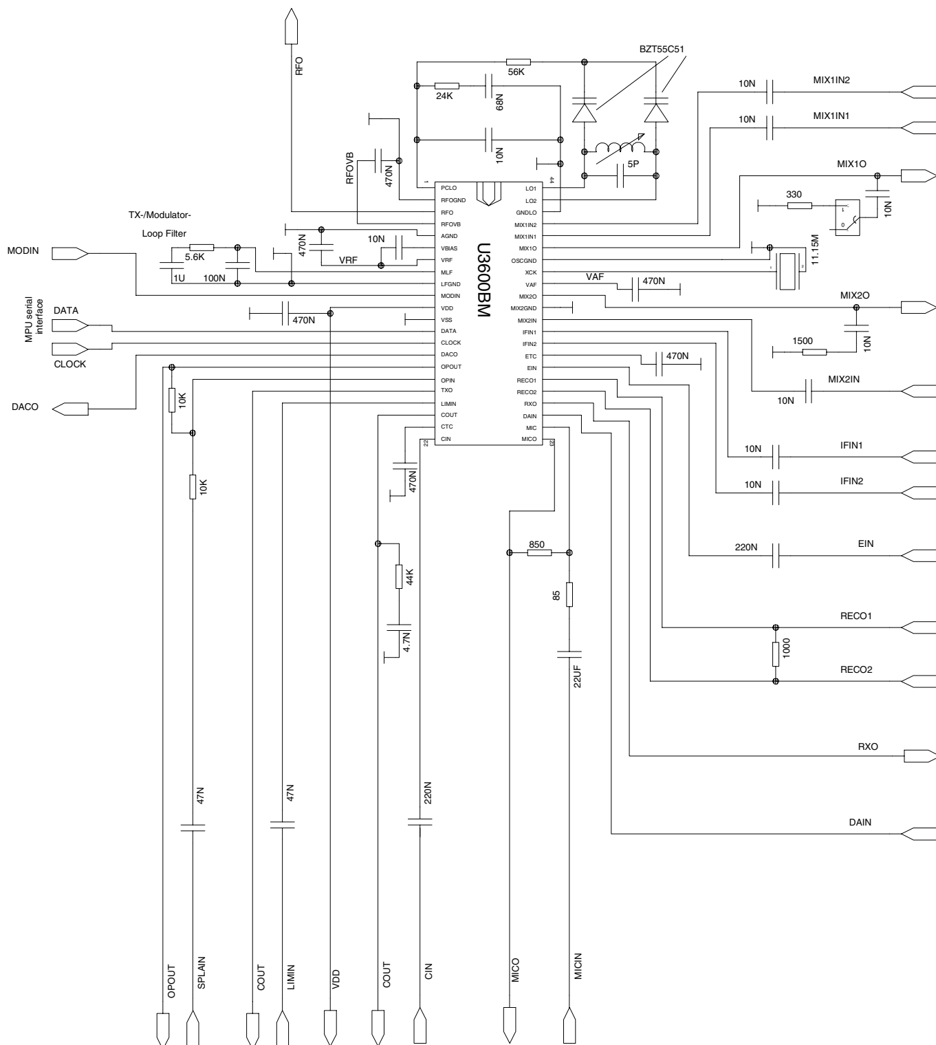
Figure 8-1. Test Circuit
