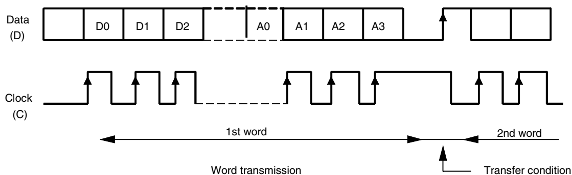
Figure 3-3. Serial Bus Structure
