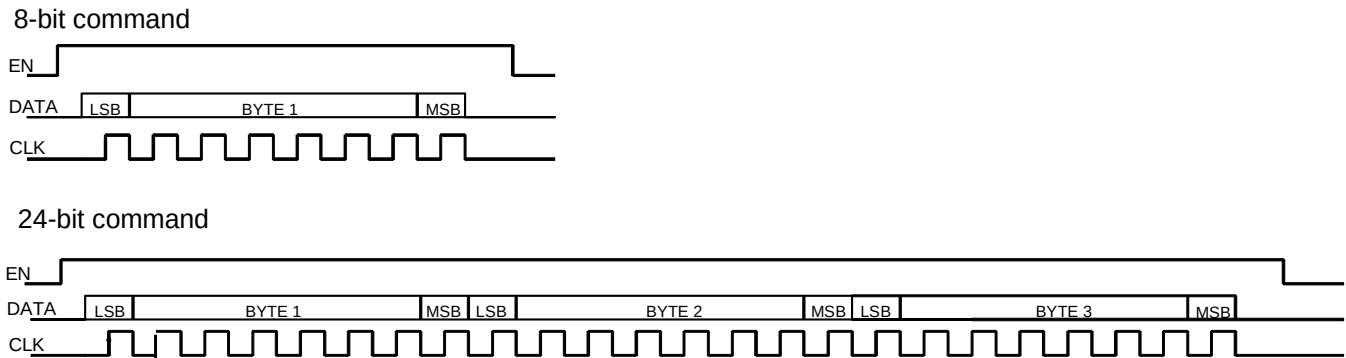
Figure 10. Pulse Diagram
