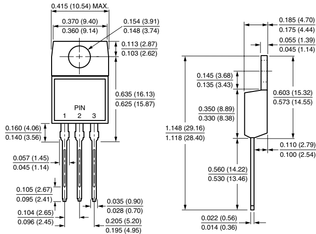
TO-220AB
