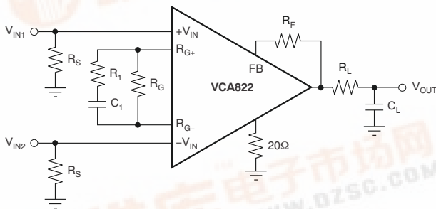
Figure 1. Differential Equalizer
