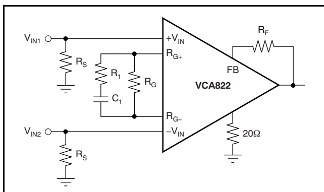
Figure 82. Differential Equalizer
