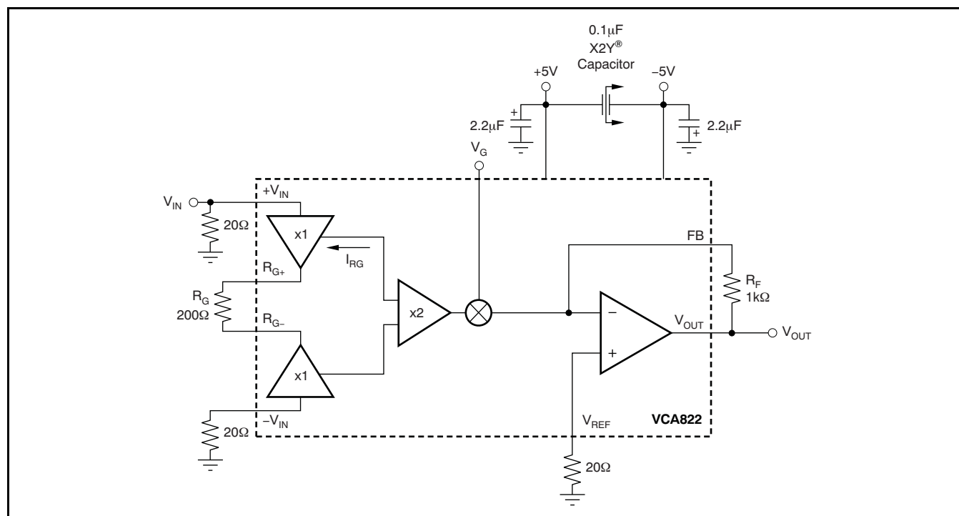
Figure 77. DC-Coupled, A_{VMAX} = +10\text{V/V} , Bipolar Supply Specification and Test Circuit
