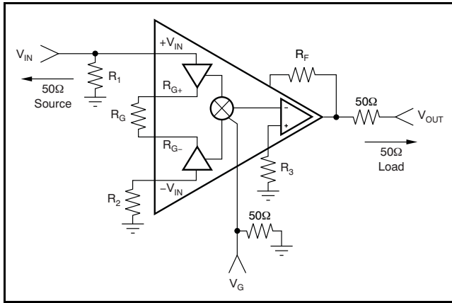
Figure 88. Test Circuit
