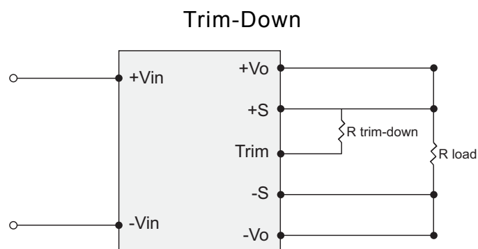
FIGURE 5: TRIM-DOWN VOLTAGE SETUP
