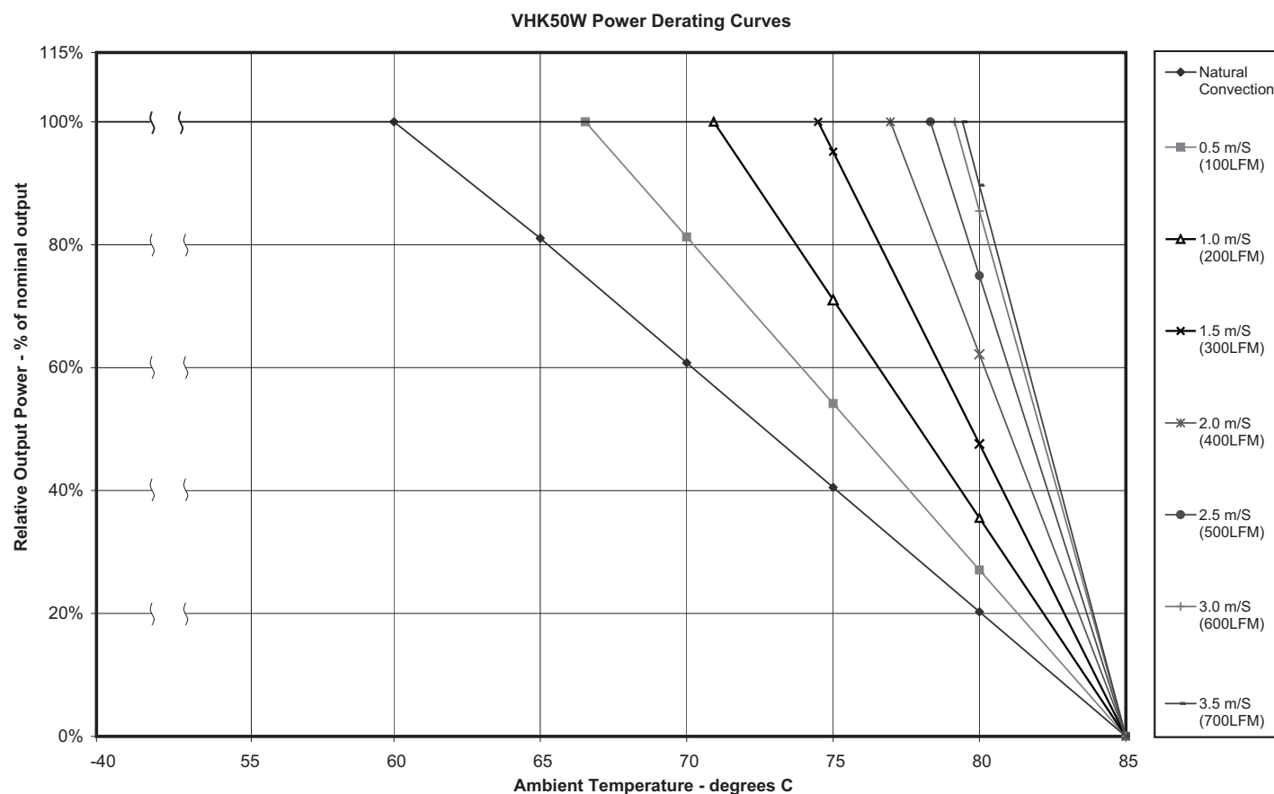
FIGURE 1. OUTPUT DERATING
