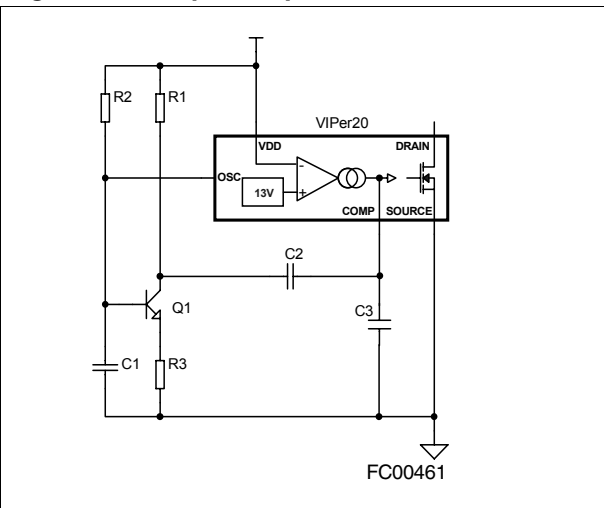
Figure 20. Slope compensation
