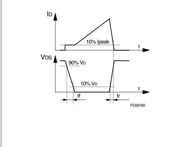
Figure 7. Transition time
