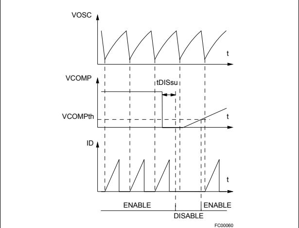
Figure 8. Shutdown action
