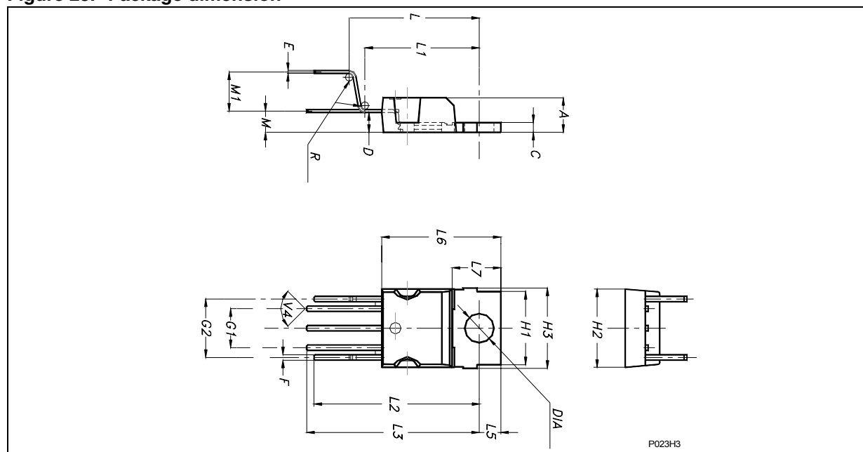
Figure 25. Package dimension
