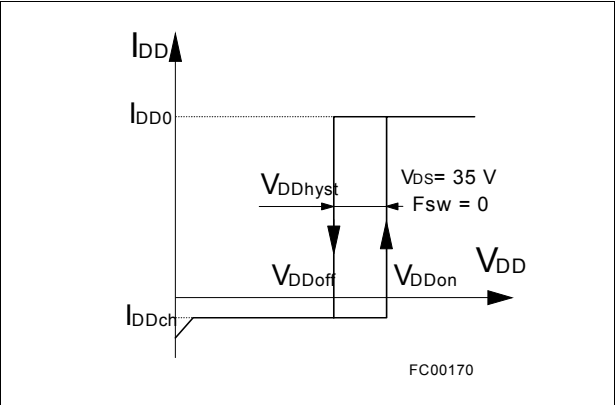
Figure 6. Undervoltage lockout
