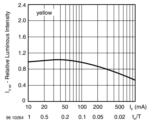
Figure 4. Rel. Lumin. Intensity vs. Forw. Current/Duty Cycle
