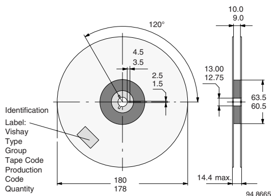
Figure 11.Reel Dimensions - GS08
