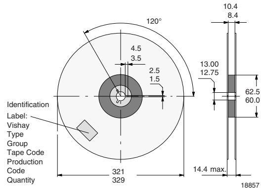
Figure 12.Reel dimensions - GS18
