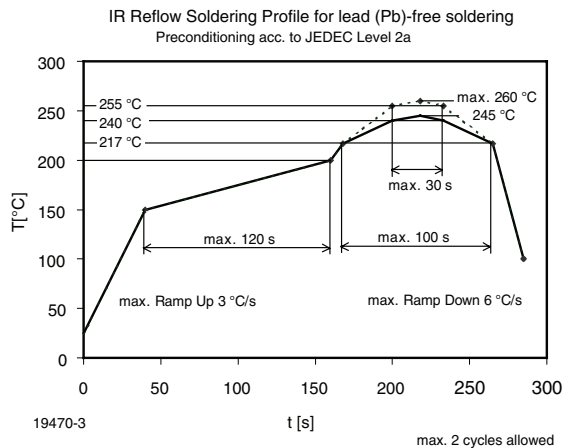
Figure 13. Vishay Lead (Pb)-free Reflow Soldering Profile (acc. to J-STD-020C)
