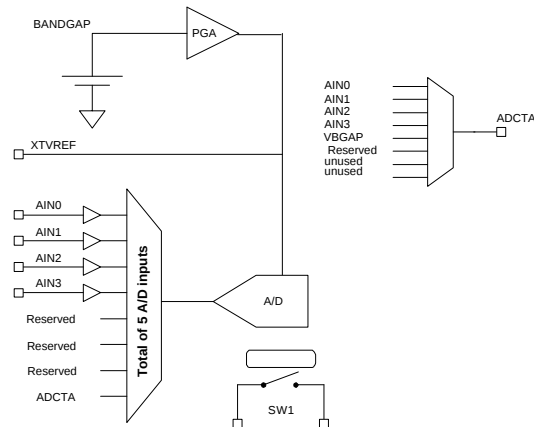
FIGURE 35: ANALOG SIGNAL PATH OF THE VMX51C1016
