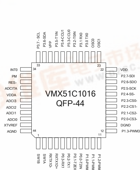
FIGURE 2: VMX51C1016-QAC14, QFP-44 PACKAGE PINOUT
