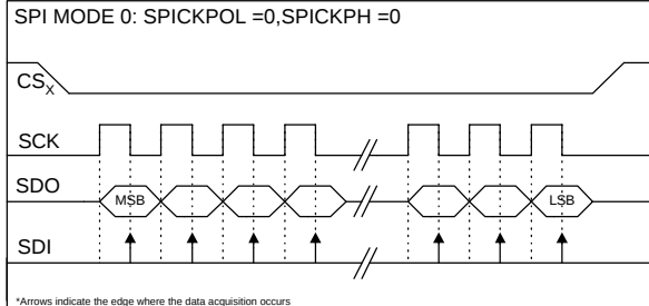
FIGURE 31 : SPI MODE 0
