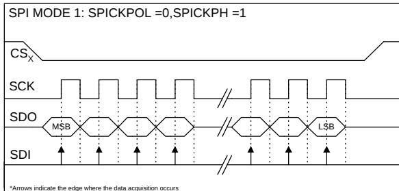
FIGURE 32: SPI MODE 1
