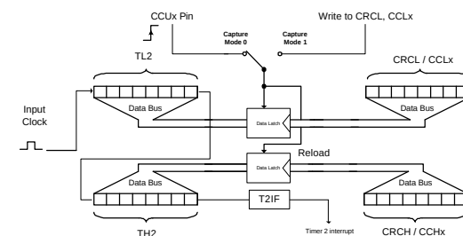
FIGURE 23:TIMER 2 CAPTURE MODE 0 FOR CBCL AND CBCH BLOCK DIAGRAM
