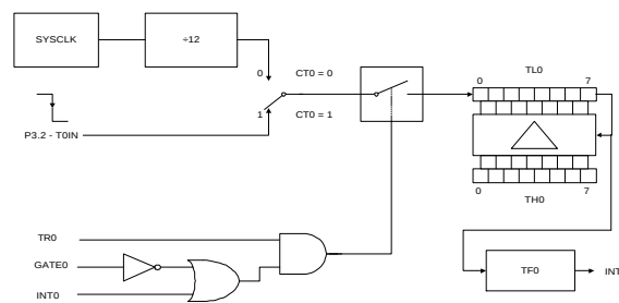
FIGURE 18 : TIMER 0 MODE 2
