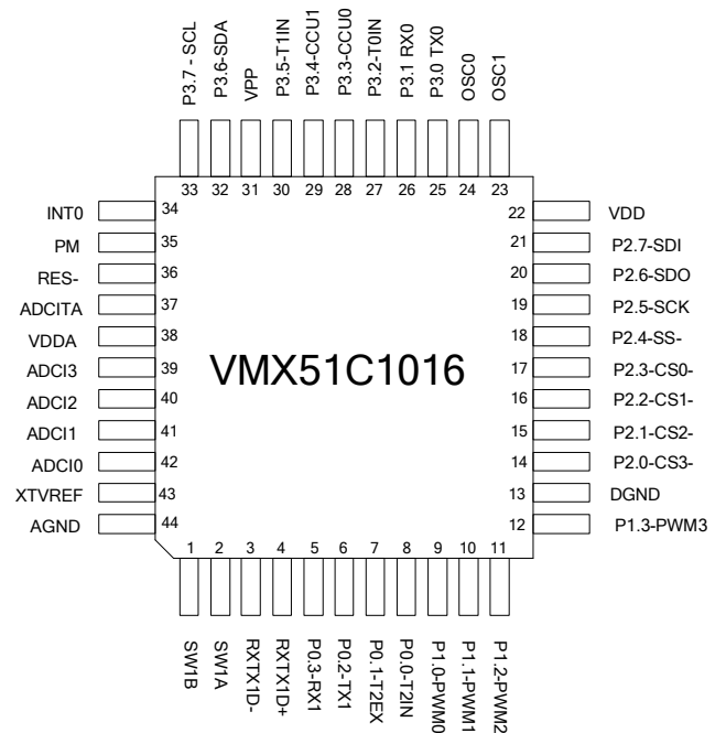
FIGURE 3: VMX51C1016 PINOUT
