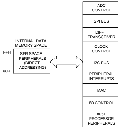
FIGURE 8: SFR ORGANIZATION
