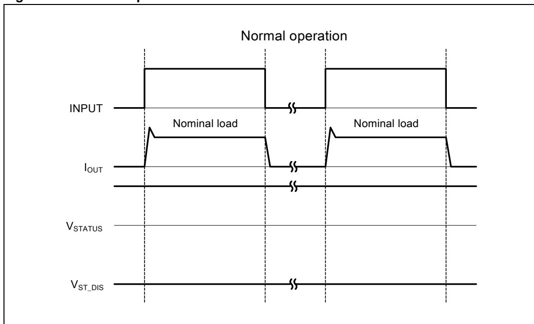
Figure 7. Normal operation
