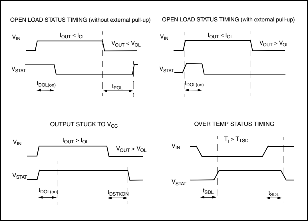
Figure 4. Status timings
