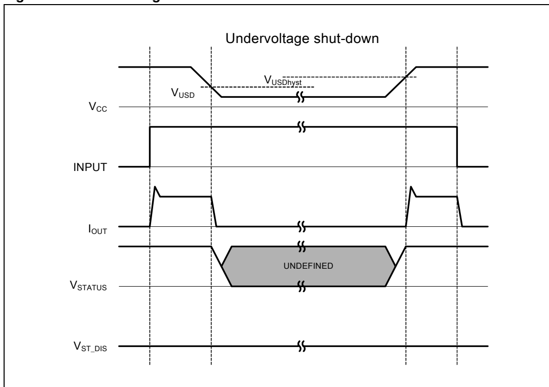
Figure 8. Undervoltage shutdown
