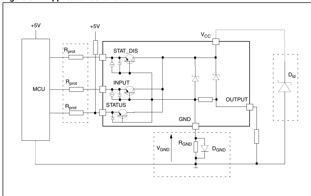
Figure 32. Application schematic
