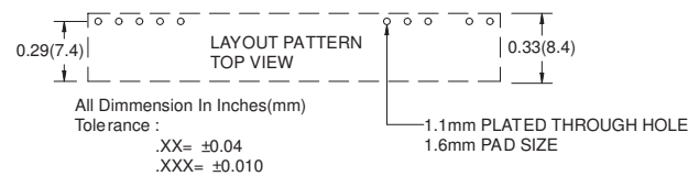
Figure 5. Recommended VPOL15A-5-SIP Footprint
