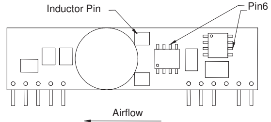
Figure 7. Temperature Measurement Location for VPOL15A-5-SIP
