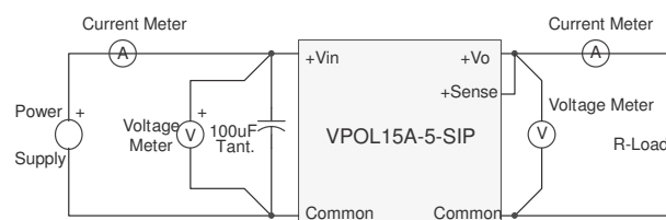
Figure 12. VPOL15A-5-SIP Series Test Setup
