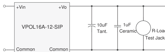
Figure 14. Output Voltage Ripple and Noise Measurement Set-Up
