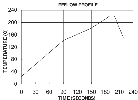
Figure 15 VPOL16A-12-SIP Reflow Profile
