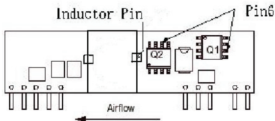
Figure 7. Temperature Measurement Location for VPOL16A-12-SIP
