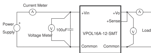
Figure 11. VPOL16A-12-SMT Series Test Setup
