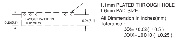
Figure 5. Recommended VPOL5A-12-SIP Footprint
