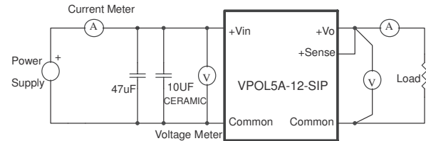
Figure 11. VPOL5A-12-SIP Test Setup
