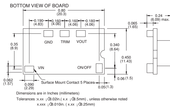
Figure 15 VPOL5A-12-SMT Mechanical Outline Diagram
